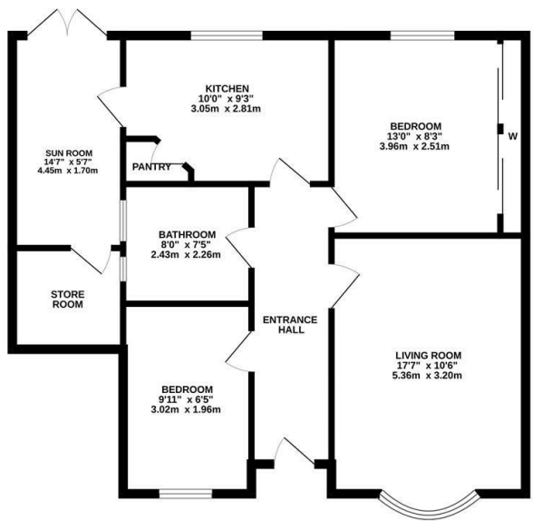
GROUND FLOOR 840 sq.ft. (78.1 sq.m.) approx.
